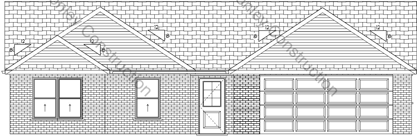
Front Elevation
