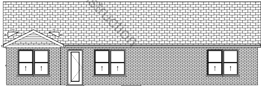
Rear Elevation
